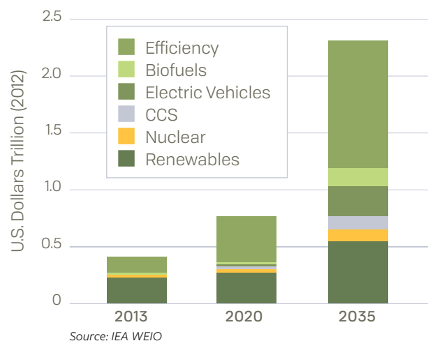
Figure 1-2. Global Investment in Low-Carbon Technologies and Energy Efficiency in the 450 Scenario.
